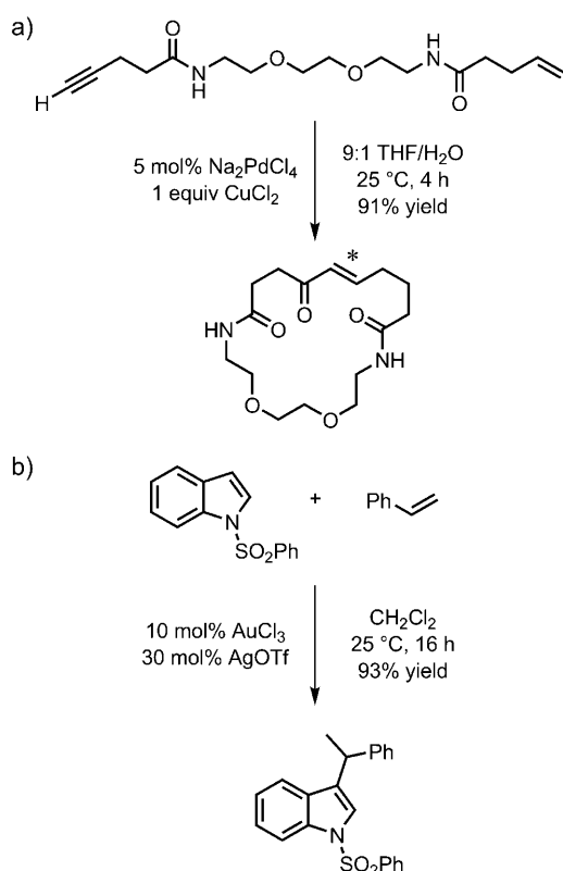
Figure 16. Examples of reactions discovered via DNA encoding. a) \text{Pd}^{\text{II}} -mediated alkene-alkyne macrocyclization reaction, discovered in hybridization-based DTS format. [76] * = site of ring closure. b) \text{Au}^{\text{III}} -mediated hydroarylation of suitably substituted alkenes with indoles, discovered in hybridization-independent (non-DTS) format. [78]
