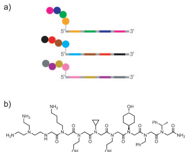
Figure 24. DNA display, in which distinct DNA sequences are used to route compounds through the combinatorial synthesis process. [110] a) Schematic depiction of three “translated” small-molecule/DNA conjugates made using four DNA “codons”. Not depicted is the split-and-pool approach used for each assembly step. b) An 8-mer peptoid ligand with K_d = 16 \mu\text{M} identified by DNA display. [111]
