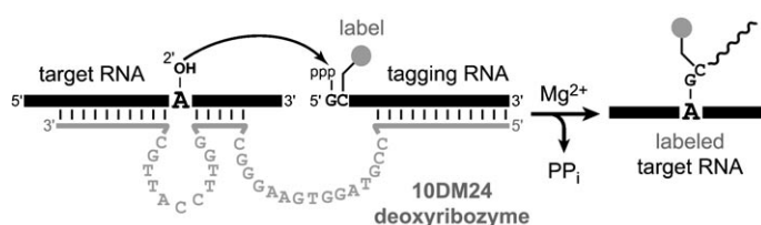
Figure 6. Deoxyribozyme-catalyzed labeling (DECAL) of RNA by the \text{Mg}^{2+} -dependent 10DM24 deoxyribozyme. [36] The label is attached to the tagging RNA as its N -hydroxysuccinimide (NHS) ester to a 5-aminoallyl group located on the nucleobase of the second nucleotide (as incorporated by in vitro transcription using 5-aminoallyl-CTP).
