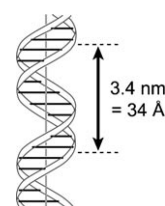
Figure 1. The DNA double helix, based upon the seminal drawing in the original Watson and Crick manuscript from 1953. [3] This structure is highly competent for long-term genetic information storage. However, catalysis by DNA requires at least partial separation of the two base-paired strands to allow formation of less regular three-dimensional structures that can support catalytic activity. Because no high-resolution structures of any catalytic DNAs are known, no analogous image of a deoxyribozyme can at present be shown.
