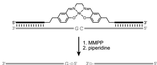
Figure 22. Example of DNA-directed catalysis: Site-specific oxidative DNA damage using a metallosalen-DNA conjugate and added magnesium monoperoxyphthalate (MMPP) as oxidant. [104] Treatment of the damaged DNA with piperidine leads to strand scission.
