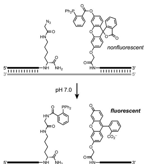
Figure 20. Staudinger reduction to activate a fluorescein fluorophore, as a representative example of nucleic acid detection via DTS. [93]
